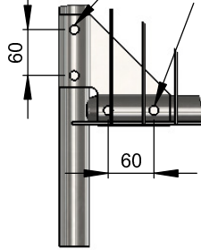
DETAIL B SCALE 2 : 12.5
