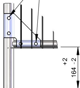
DETAIL A SCALE 2 : 12.5
