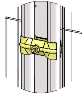
VIEW ON BACK FACE SHOWING VERTICAL BOARD FIXING WITH COUPLER 08551030
