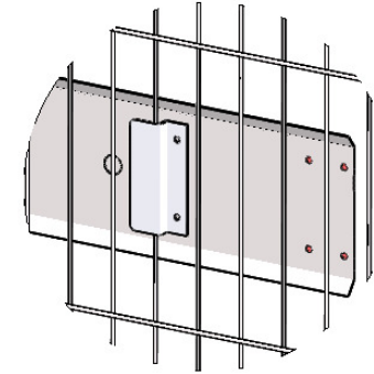
VIEW ON BACK FACE SHOWING HORIZONTAL BOARD FIXING WITH BRACKET 02251620
