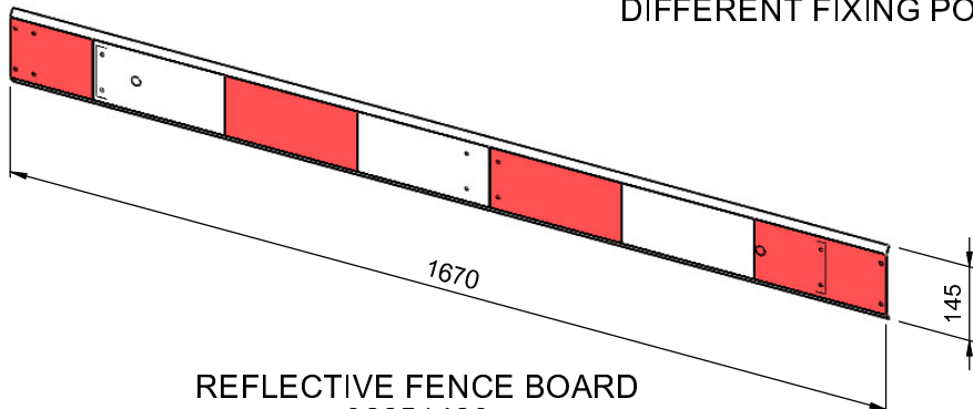
VIEW ON FRONT FACE SHOWING DIFFERENT FIXING POSITIONS
