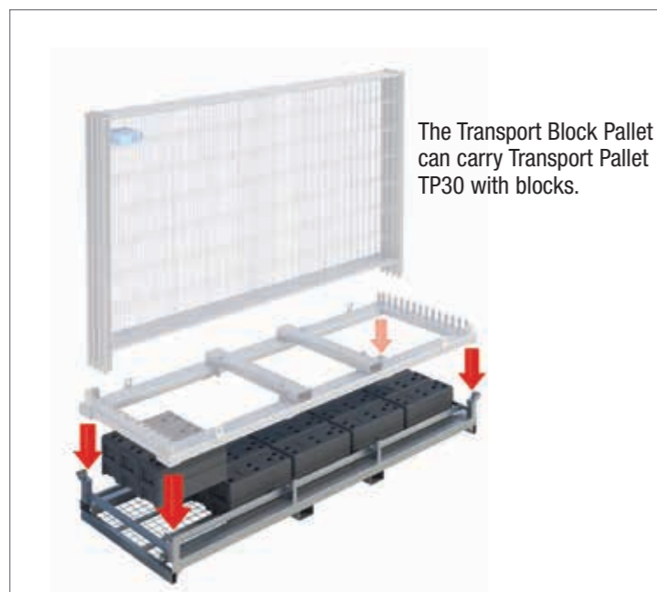
Transport Block Pallet Code: 20025 Weight: 159Kg Finish: Post Galvanised
