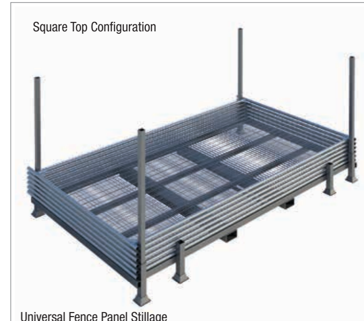
Universal Fence Panel Stillage Code: 20060 Weight: 204Kg Finish: Post Galvanised
