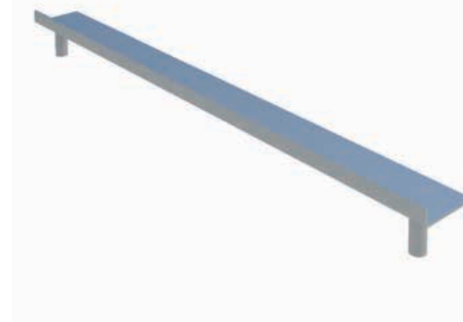
Transport Pallet 30 Spreader Bar Code: 20064 Weight: 7.5kg Finish: Pre Galvanised
