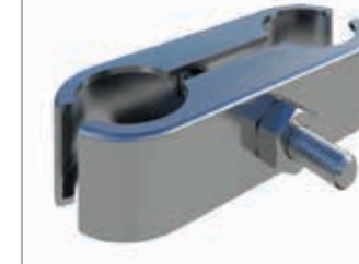
F H B Heavy Duty Fence Coupler (Gripper) Code: 20002 Weight: 0.4kg Finish: Electro Galvanised
