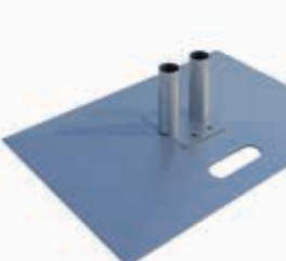
F H B Large Foot Plate – Euro Code: 20068 Weight: 12.5Kg Finish: Electro Galvanised
